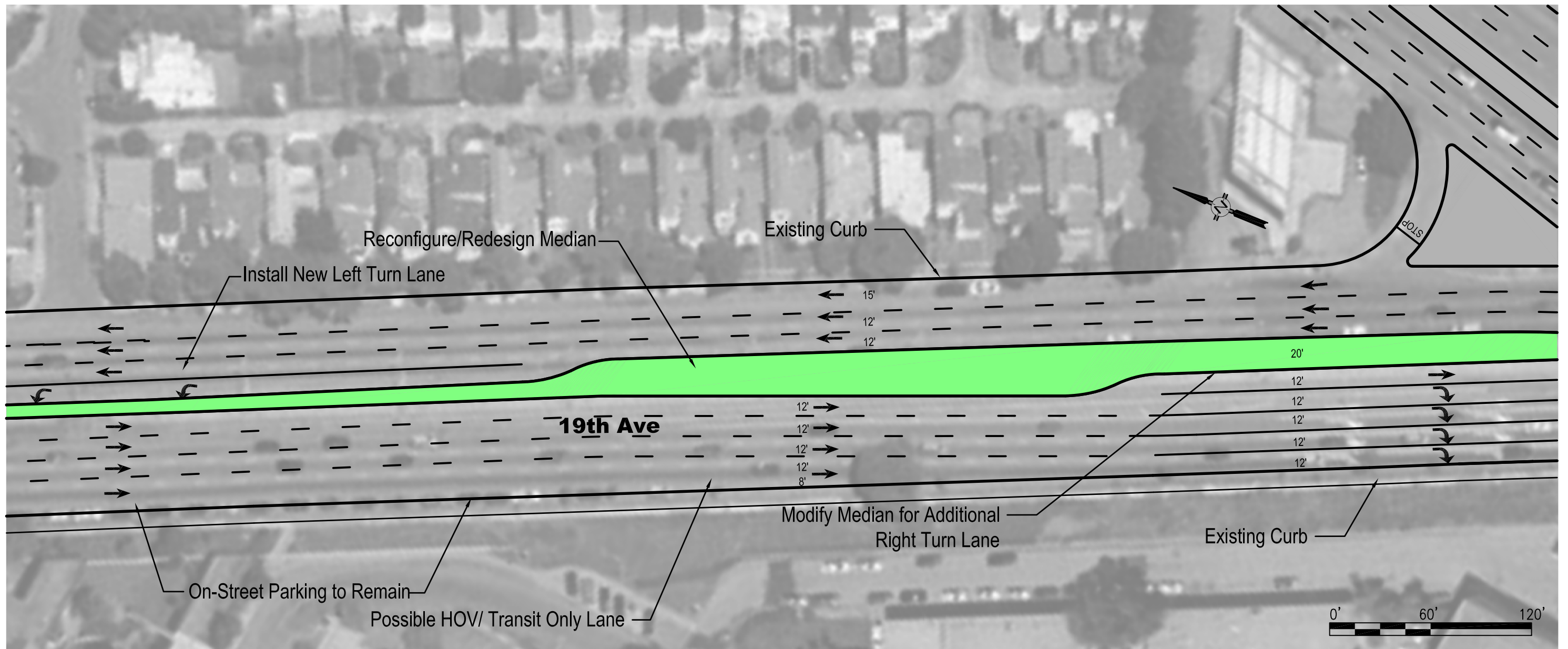
19TH AVENUE BETWEEN CRESPI DRIVE AND JUNIPERO SERRA BOULEVARD Tier 4C
