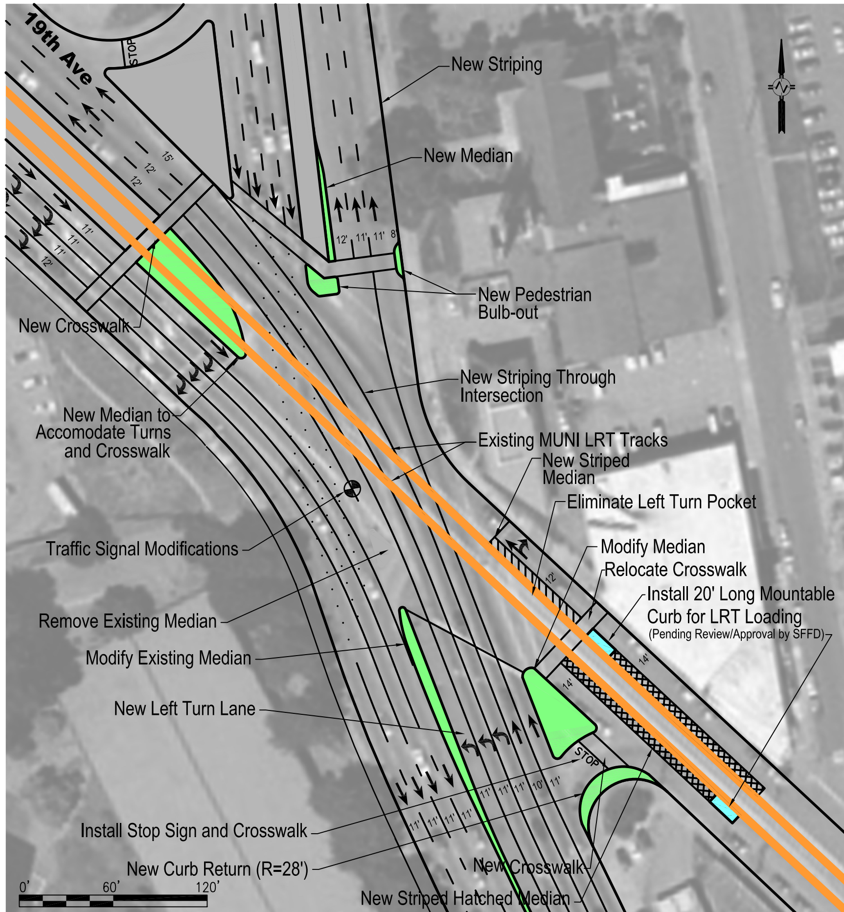
19TH AVENUE / JUNIPERO SERRA BOULEVARD Tier 4A
