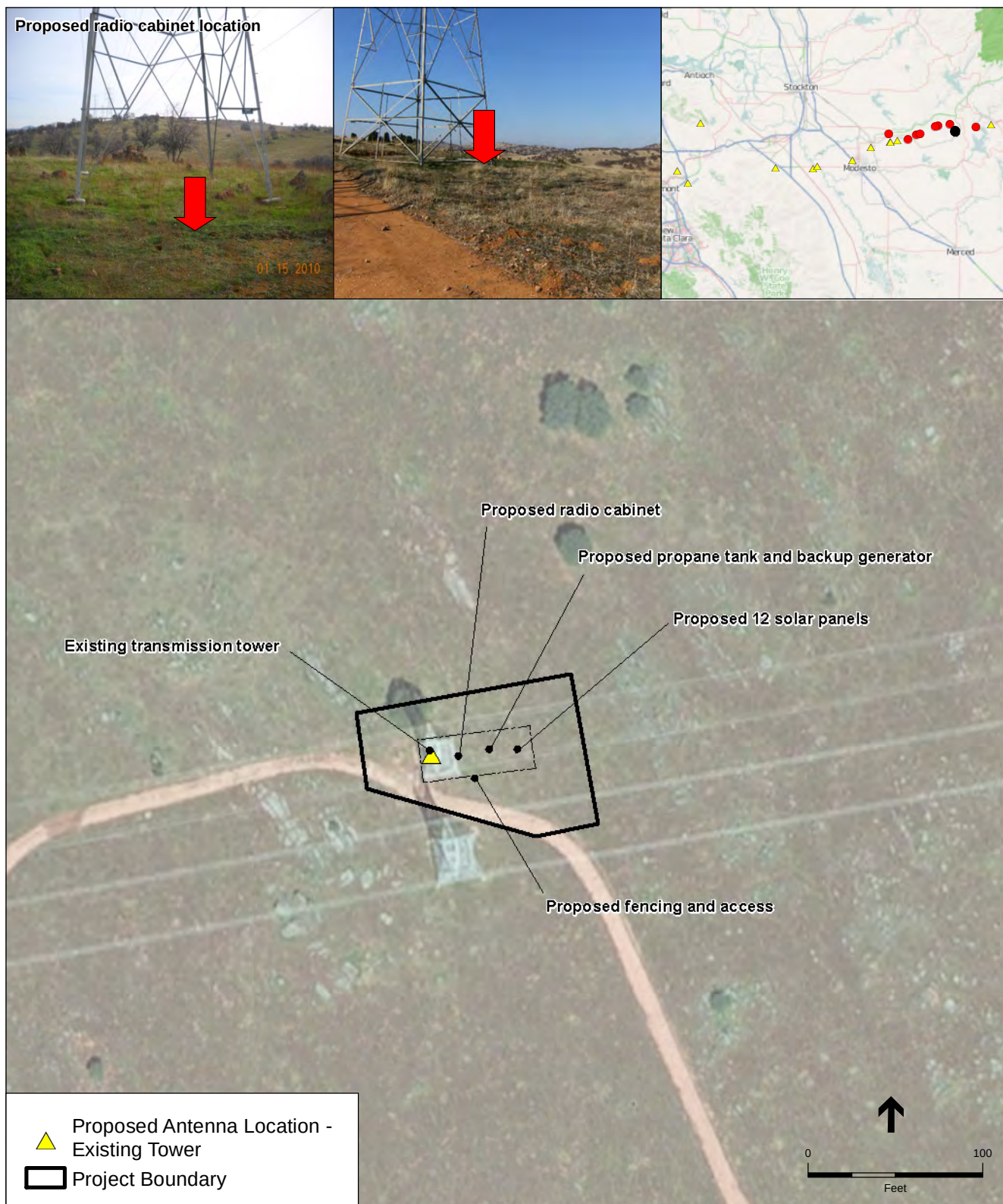
Figure 2-3 Transmission Tower 122N (Site 3)
