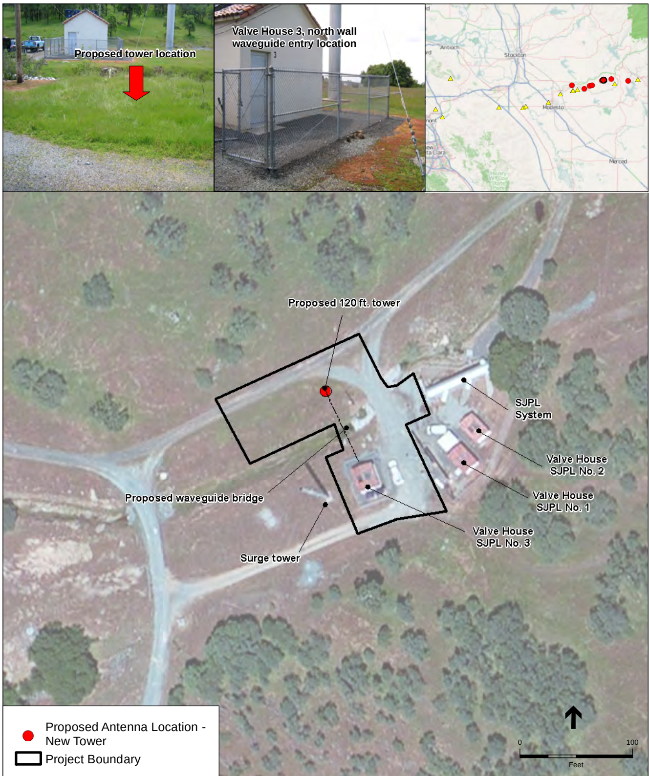
Figure 2-5 Oakdale Portal (Site 5)
