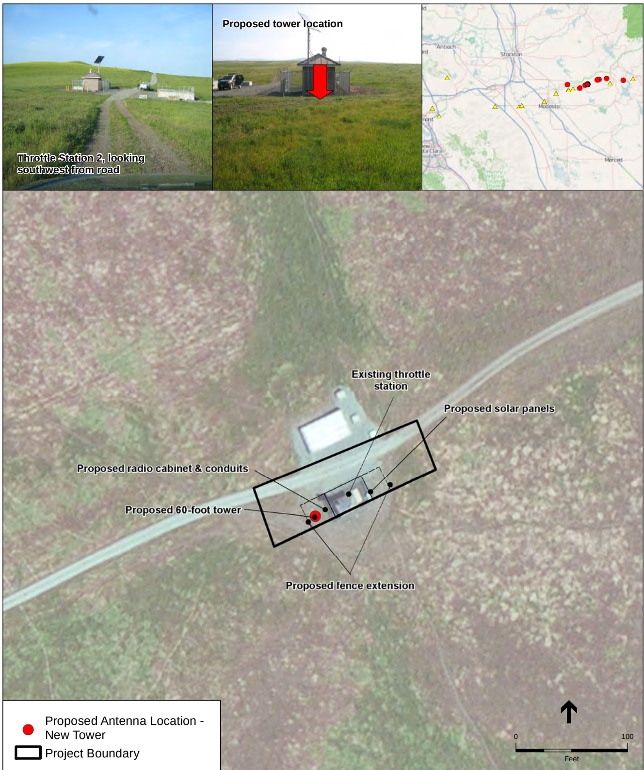
SOURCE: ESRI, 2011; Goodman Networks San Joaquin Valley Communication System Upgrade Project Figure 2-7 Throttle Station 2 (Site 7)
